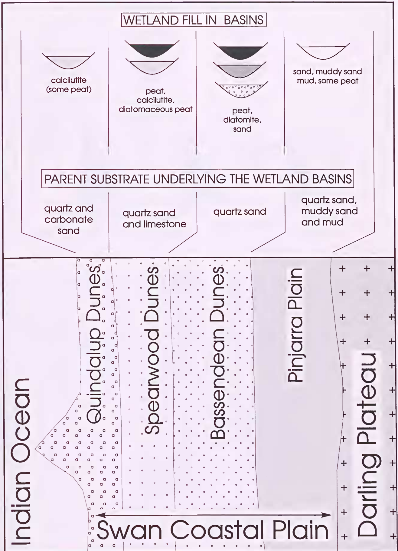
Figure 12. Idealised diagram summarising, with respect to geomorphic setting across the Swan Coastal Plain, the distribution of parent substrate types underlying wetland basins and the (simplified) wetland sediment types in basins.
